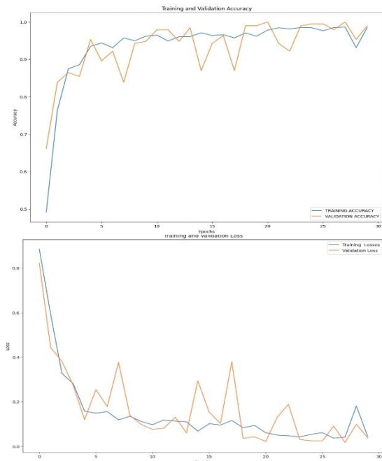
Fig. 5: Training and Validation Accuracy
