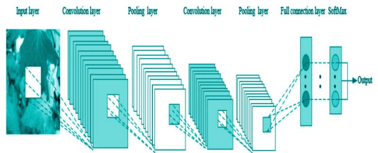
Fig.2: Basic Structure of CNN
